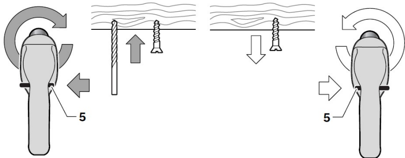
(2) Forward/Reverse lever
